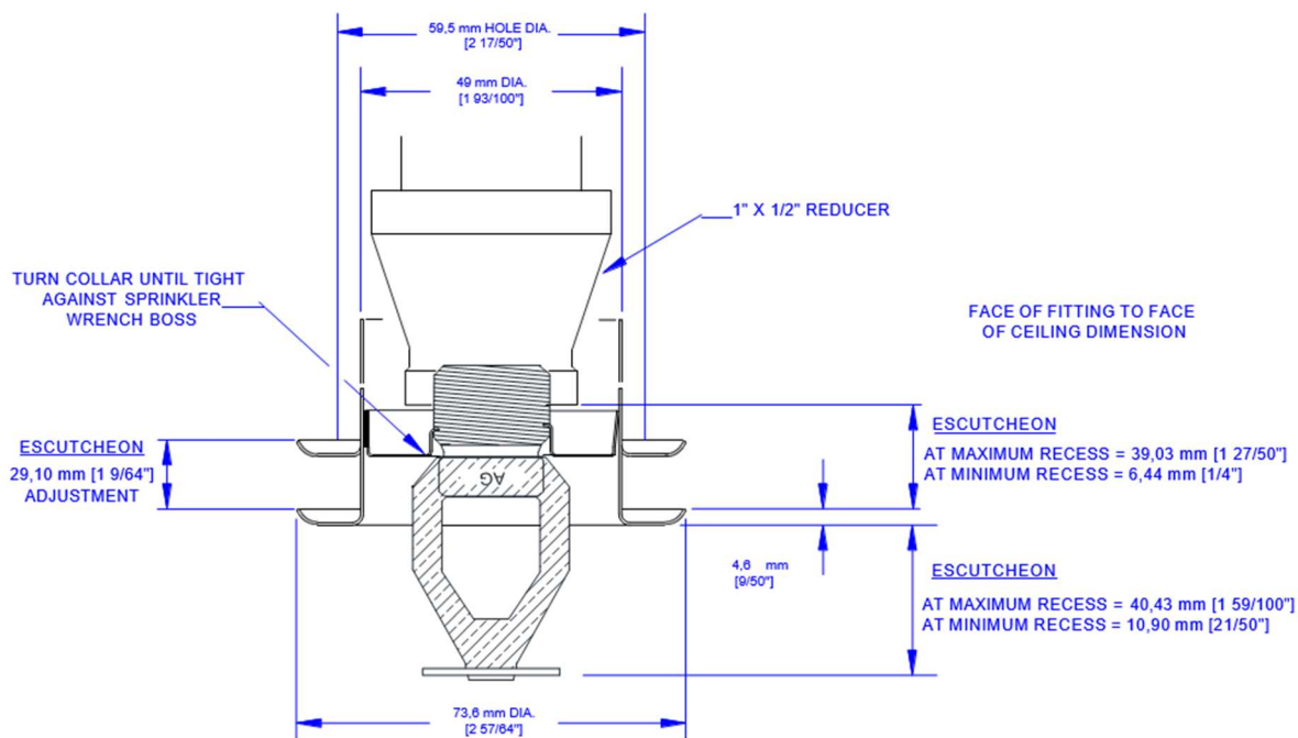
RECESSED PENDENT
