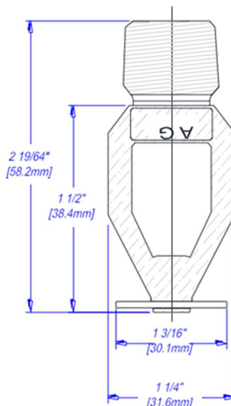
PENDENT
